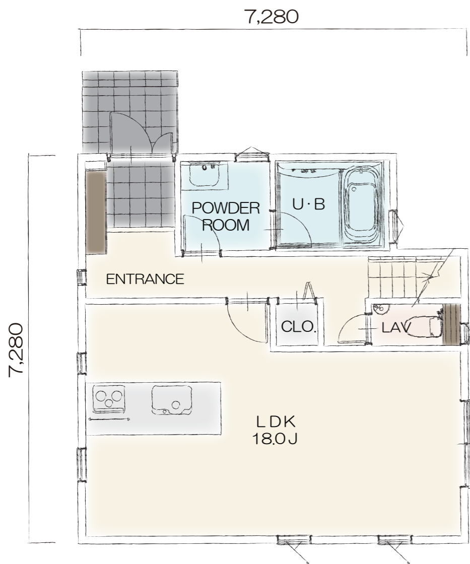
1F PLAN
