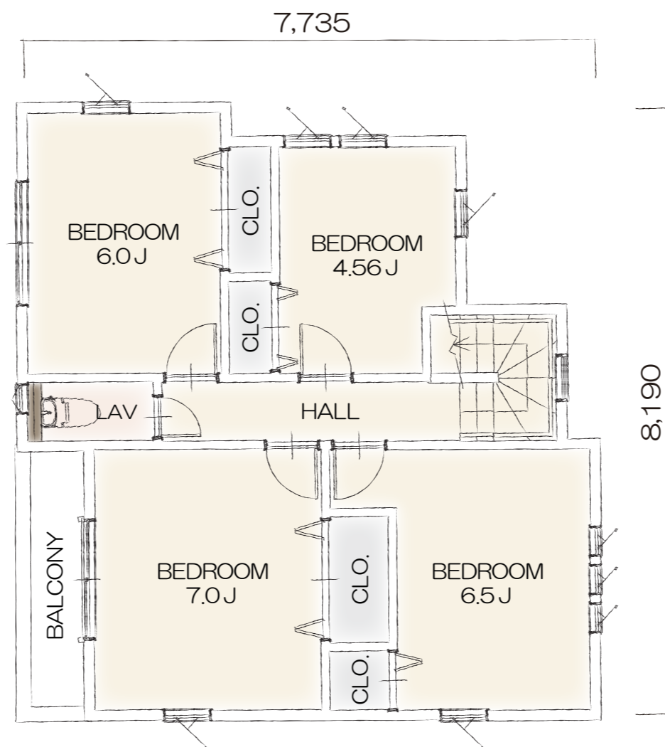
2F PLAN
