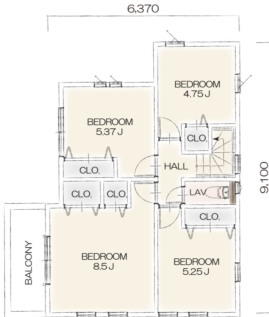
2F PLAN
