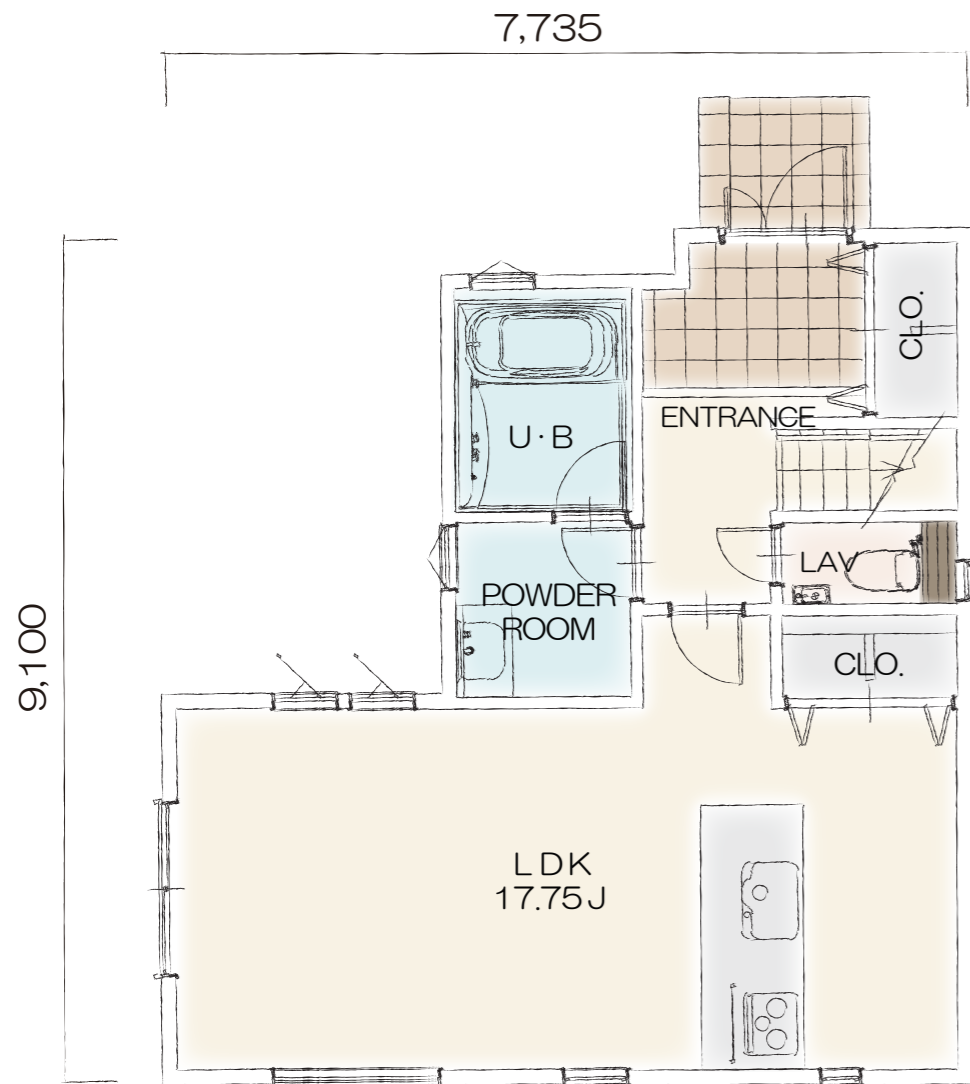
1F PLAN
